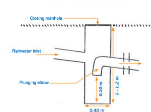
SETTLING SUMP
